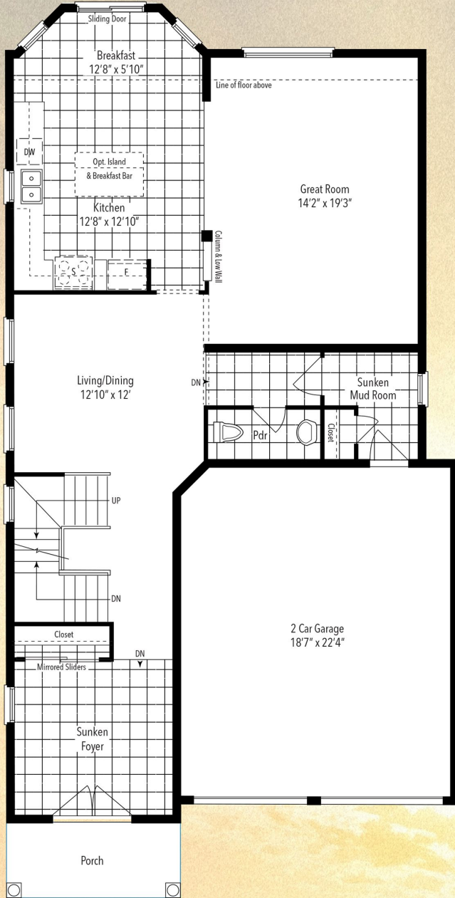
1st Floor
