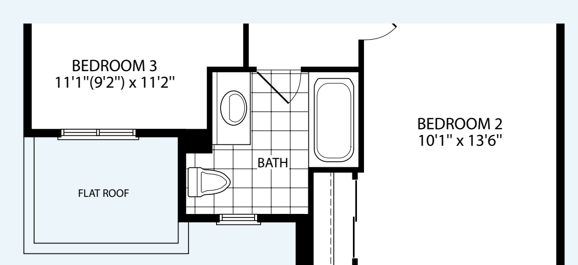
SECOND FLOOR ELEV. B
