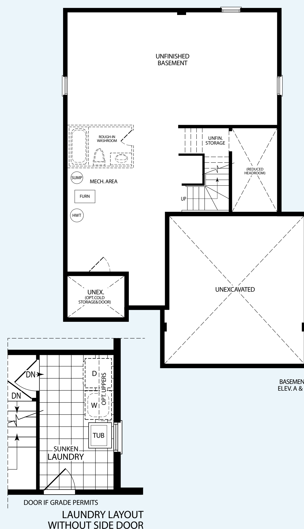
LAUNDRY LAYOUT WITHOUT SIDE DOOR
