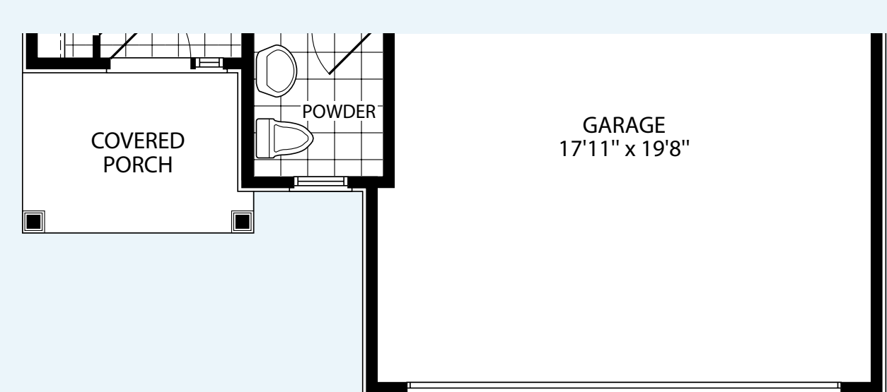
FIRST FLOOR ELEV. B
