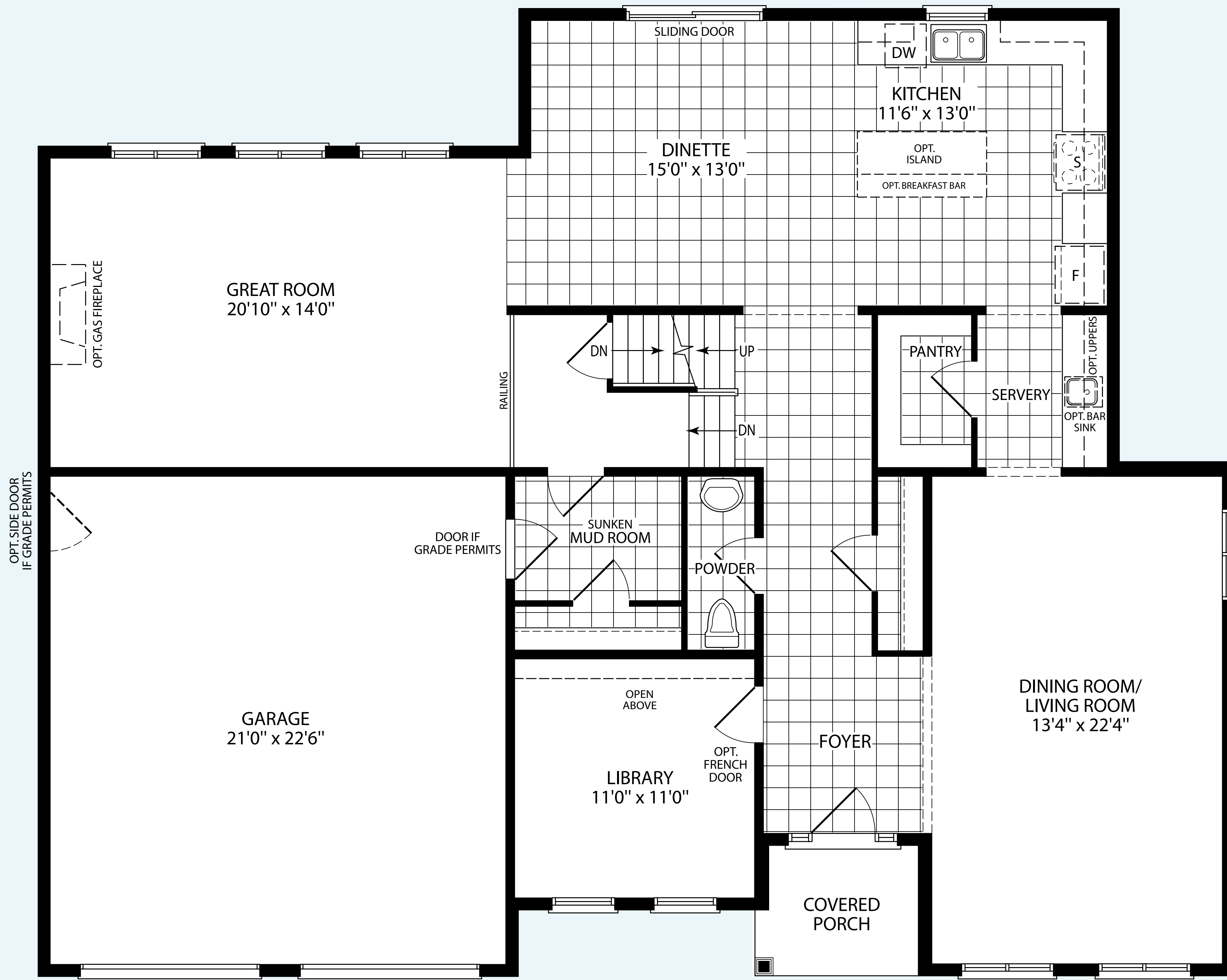
FIRST FLOOR ELEV. A
