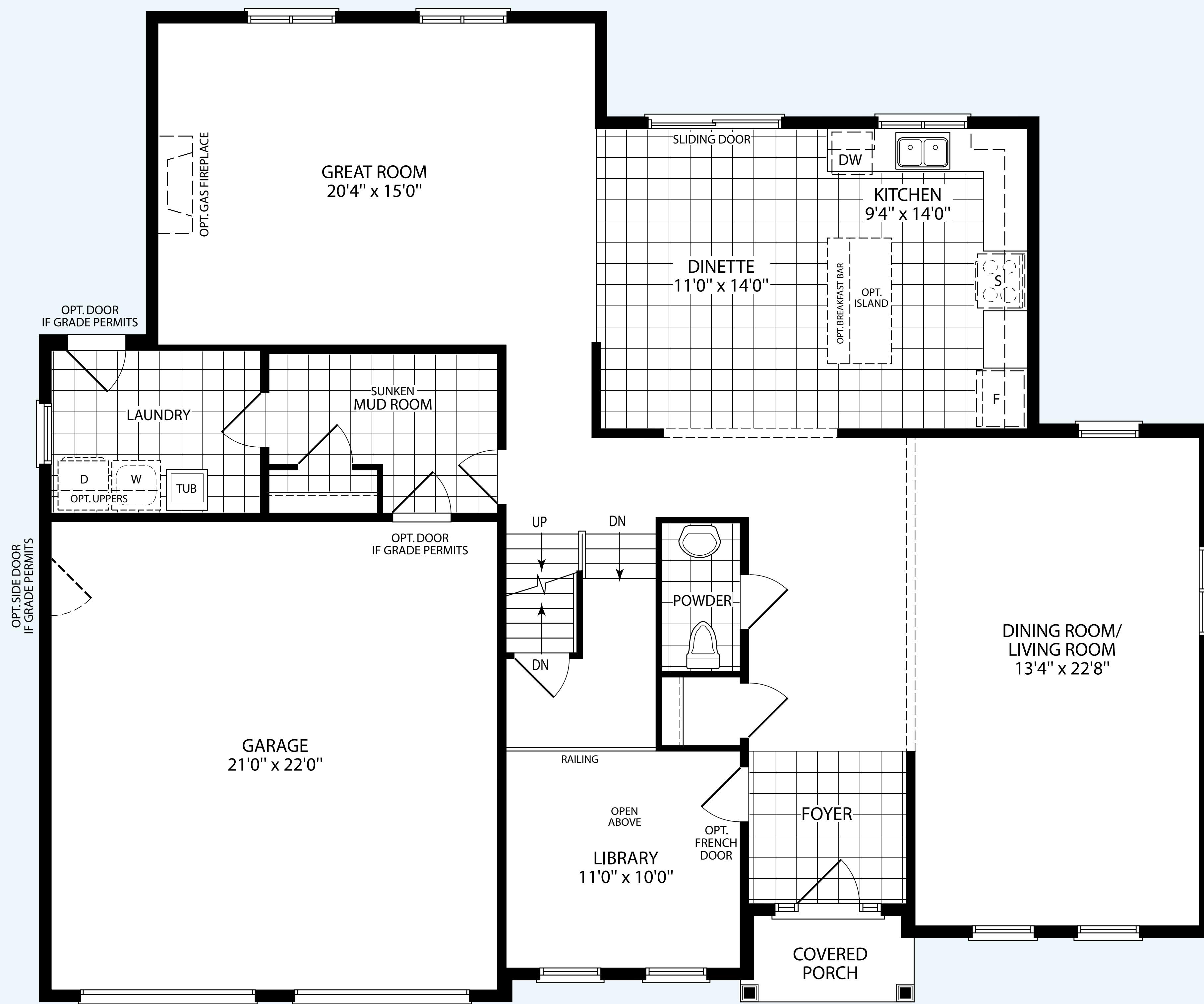
FIRST FLOOR ELEV. A
