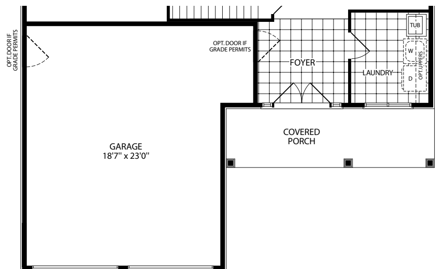
FIRST FLOOR ELEV. B
