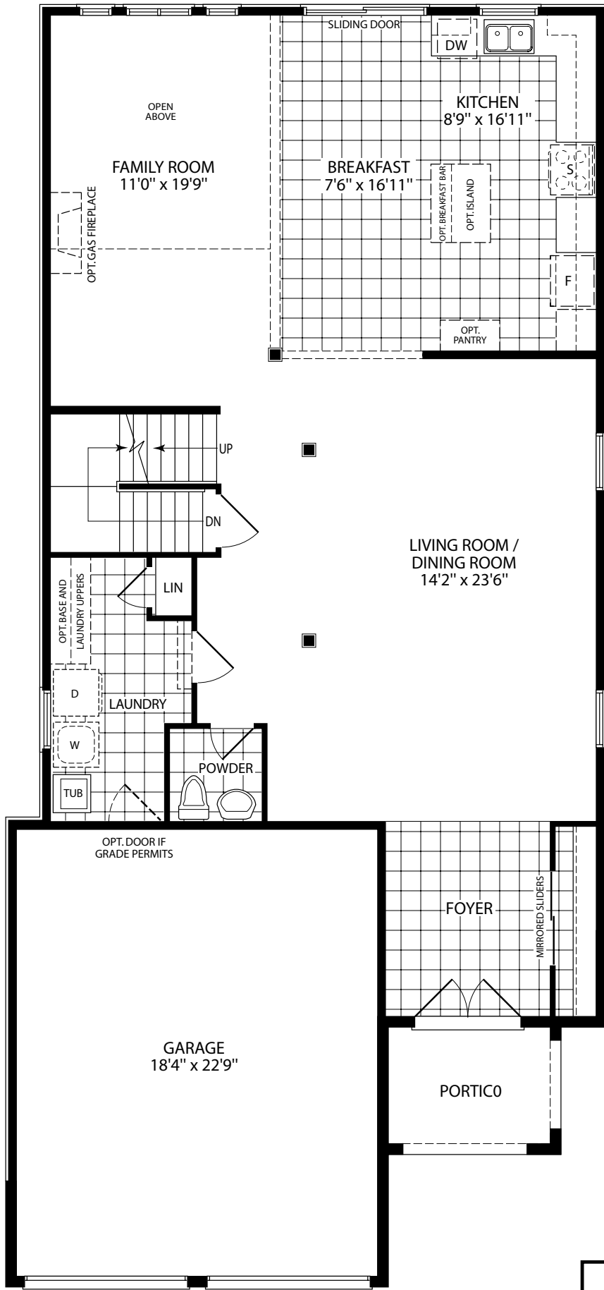
FIRST FLOOR ELEV. A
