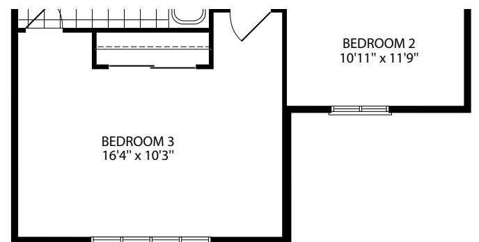
SECOND FLOOR ELEV. B
