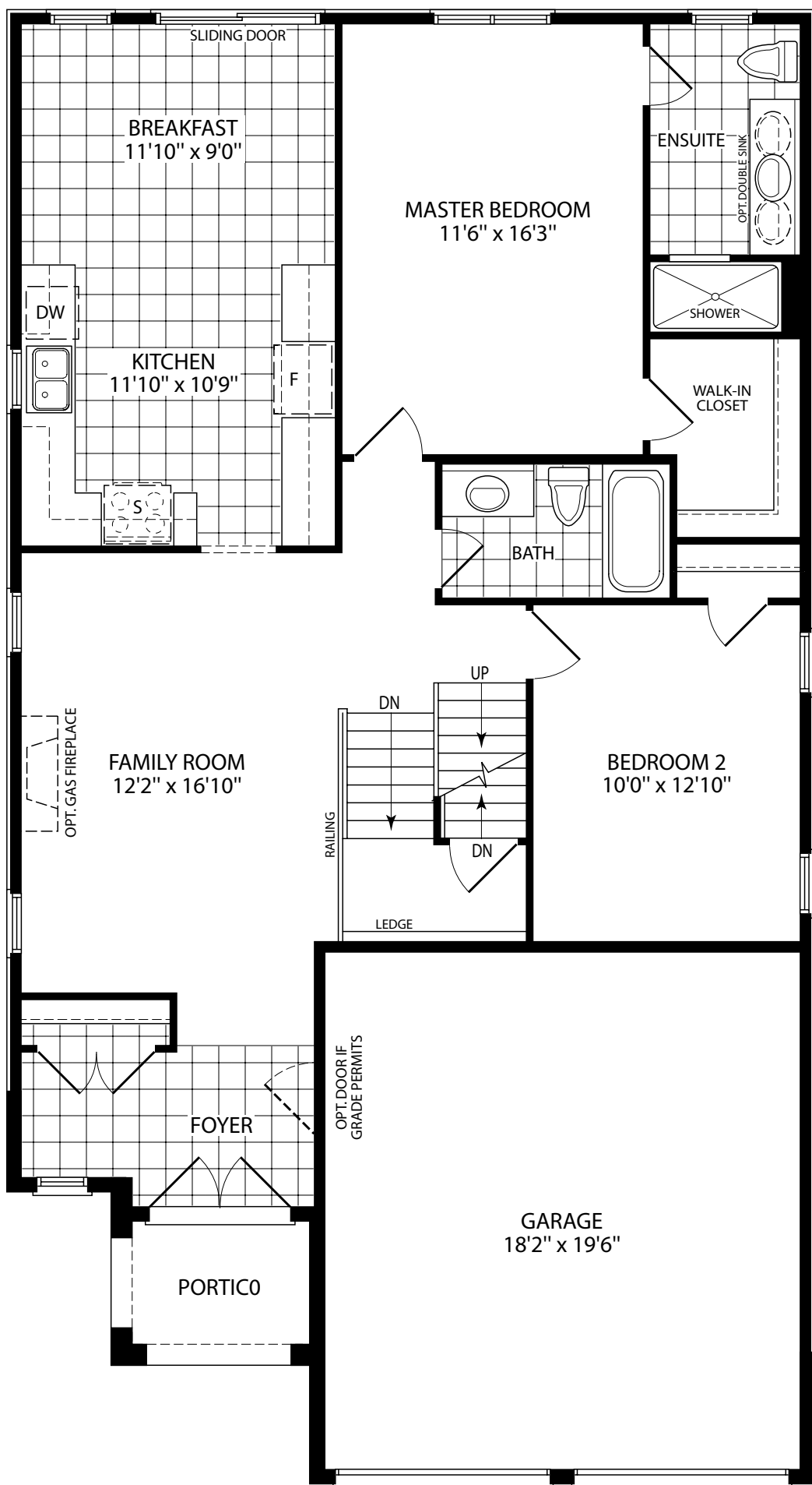
FIRST FLOOR ELEV. A
